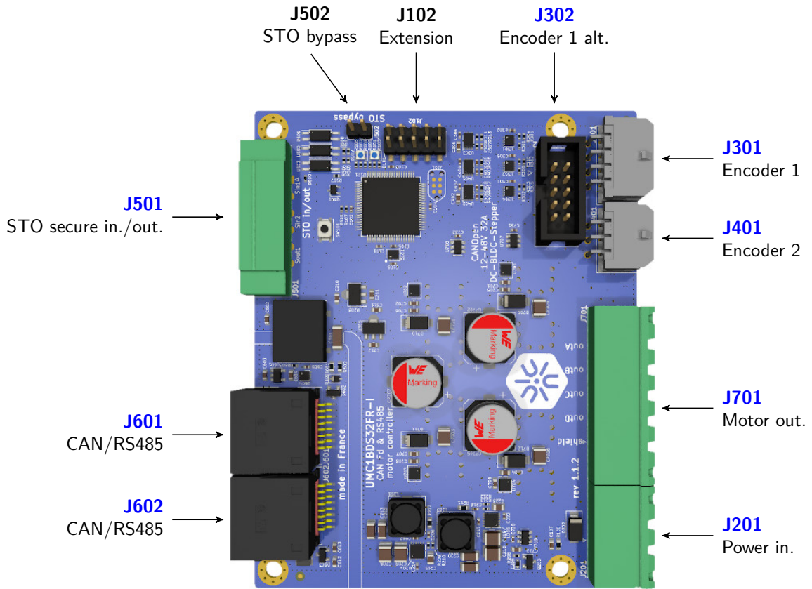
Figure 1.1: UMC1BDS32 connectors
